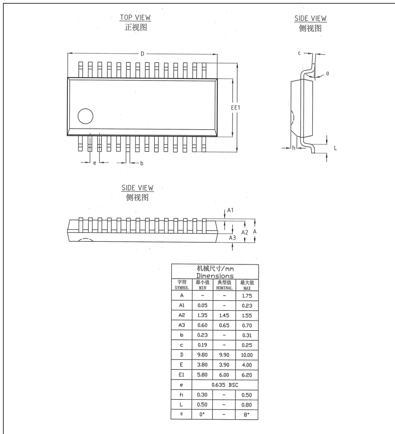
Figure 4-2 SSOP28 (0.635mm) 封装尺寸
