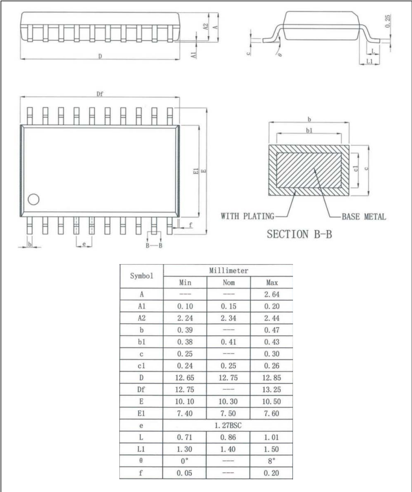
Figure 4-4 SOP20封装尺寸
