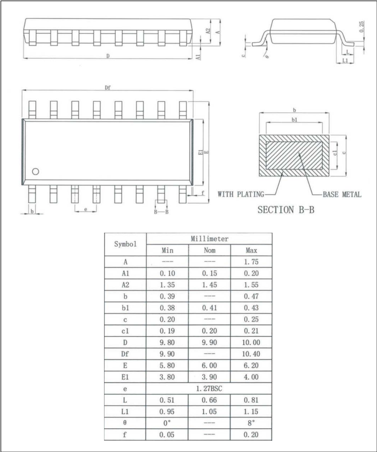
Figure 4-5 SOP16封装尺寸
