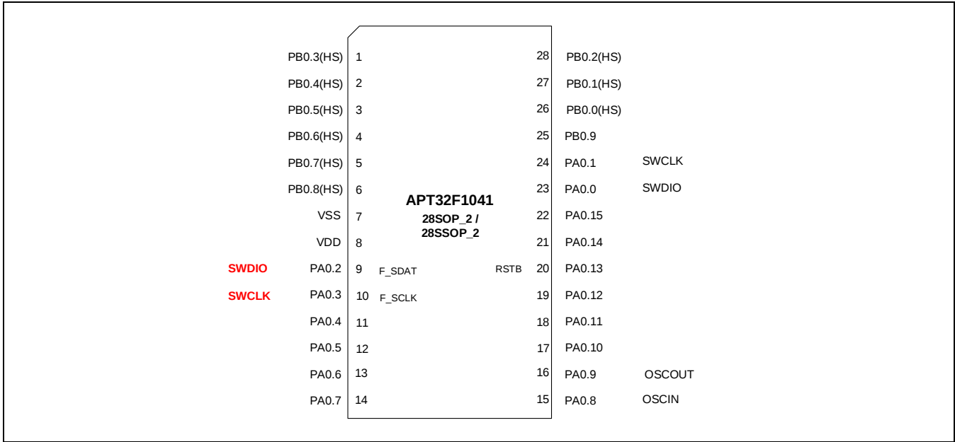
Figure 2-1 管脚定义图(SOP28_2/SSOP28_2)
