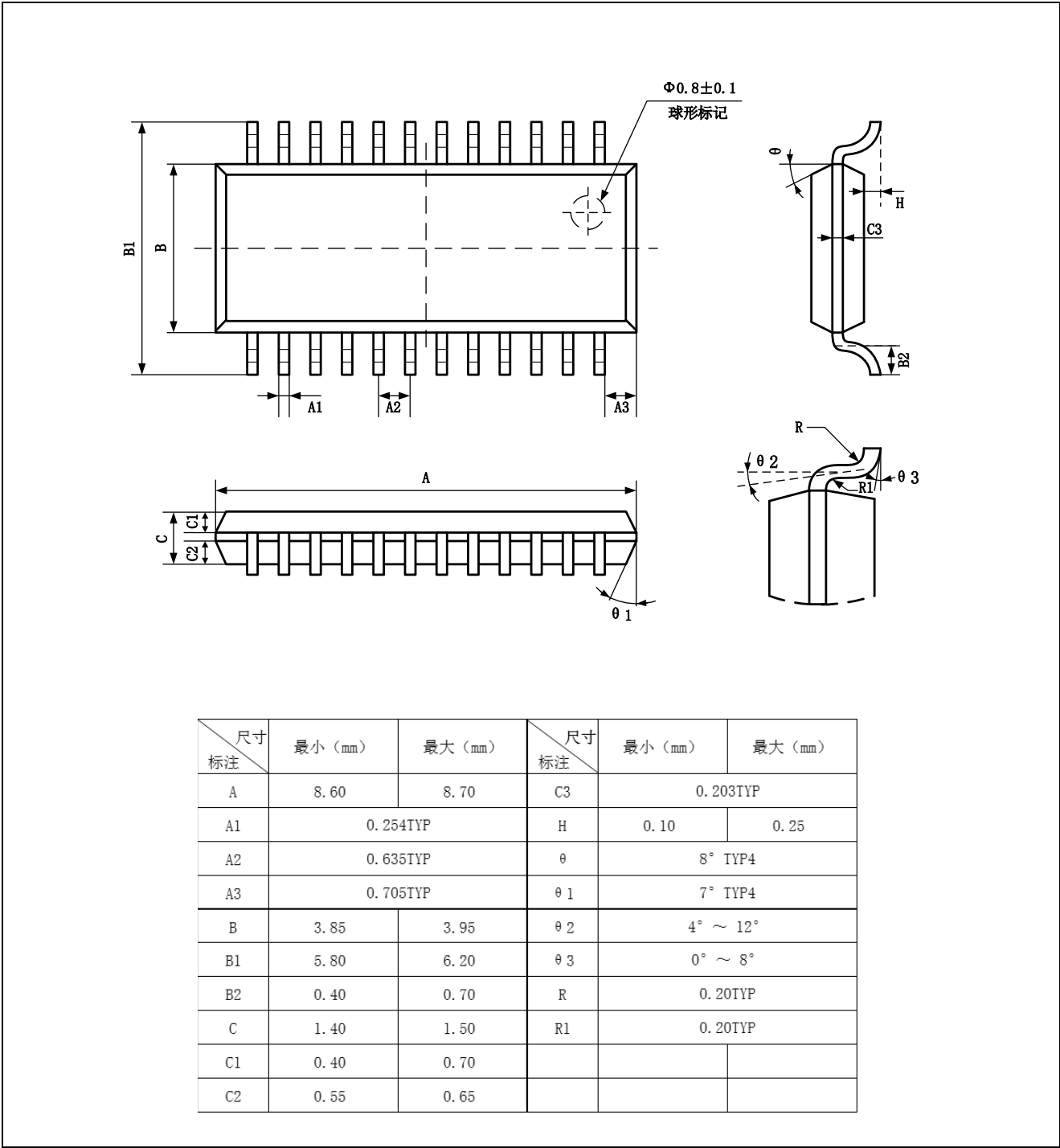
Figure 4-3 SSOP24 (0.635mm) 封装尺寸
