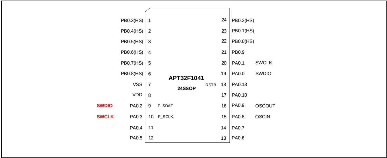
Figure 2-2 管脚定义图(SSOP24)
