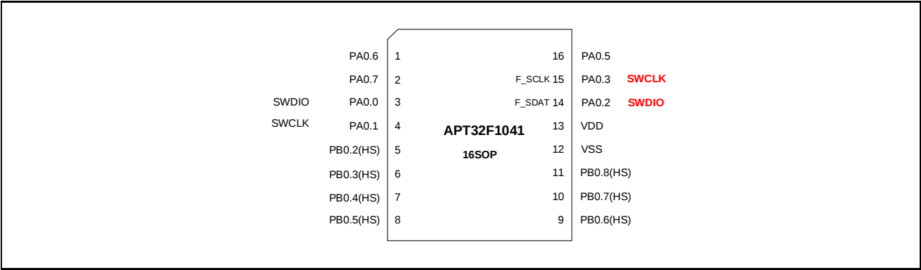
Figure 2-4 管脚定义图(SOP16)
